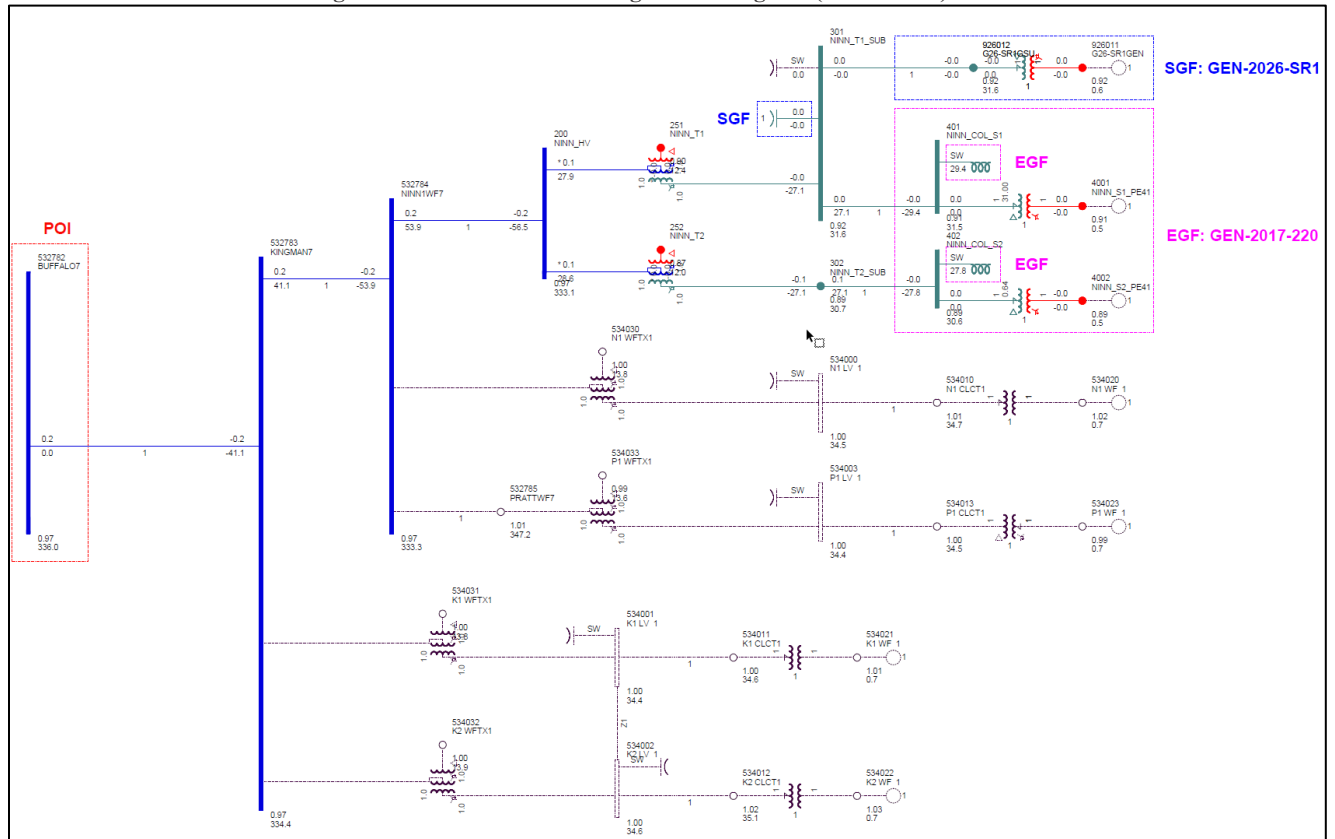
Figure 3-1: GEN-2026-SR1 Single Line Diagram (Shunt Sizes)
