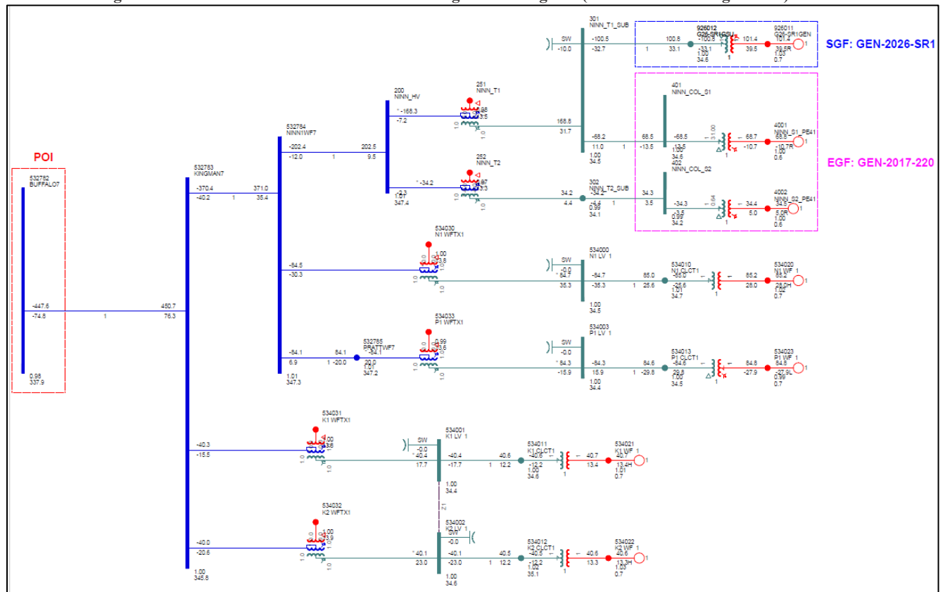
Figure 2-2: GEN-2017-220 &amp; GEN-2026-SR1 Single Line Diagram (EGF &amp; SGF Configuration)
