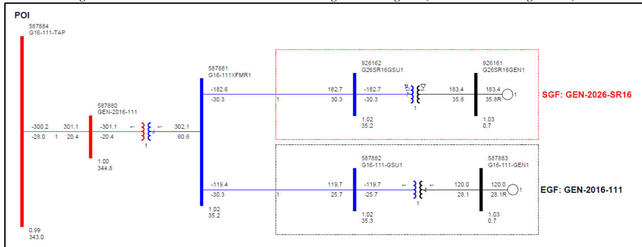
Figure 2-2: GEN-2016-111 & GEN-2026-SR16 Single Line Diagram (EGF & SGF Configuration)
