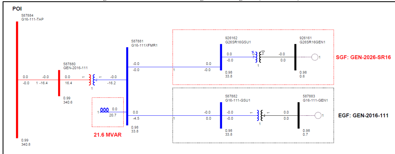
Figure 3-1: GEN-2026-SR16 Single Line Diagram (Shunt Sizes)
