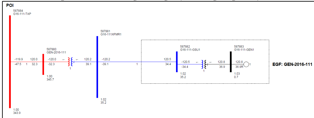
Figure 2-1: GEN-2016-111 Single Line Diagram (EGF Existing Configuration*)
