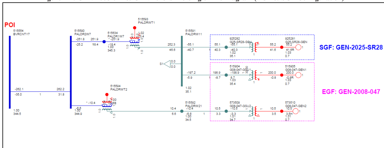
Figure 2-2: GEN-2008-047 &amp; GEN-2025-SR28 Single Line Diagram (EGF &amp; SGF Configuration)
