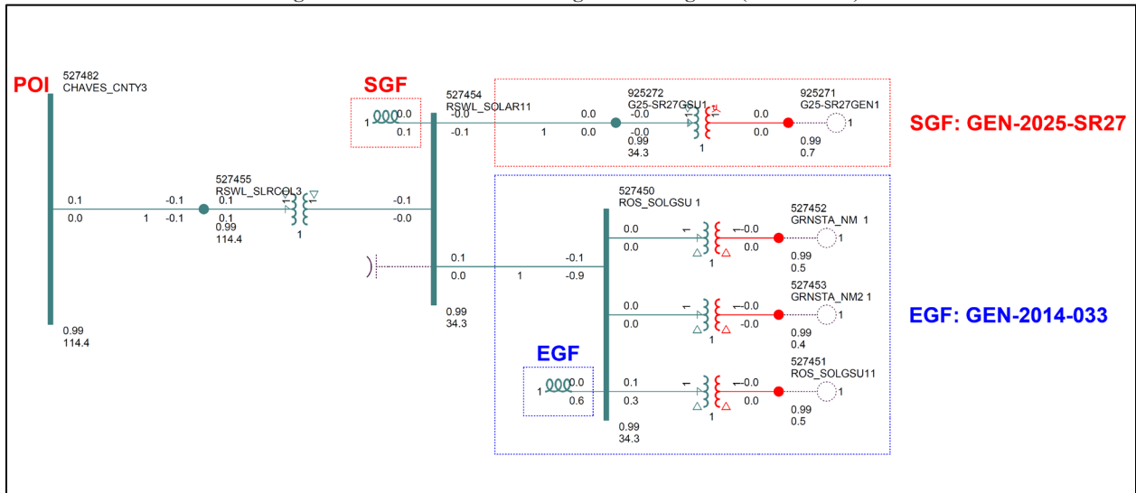
Figure 3-1: GEN-2025-SR27 Single Line Diagram (Shunt Sizes)
