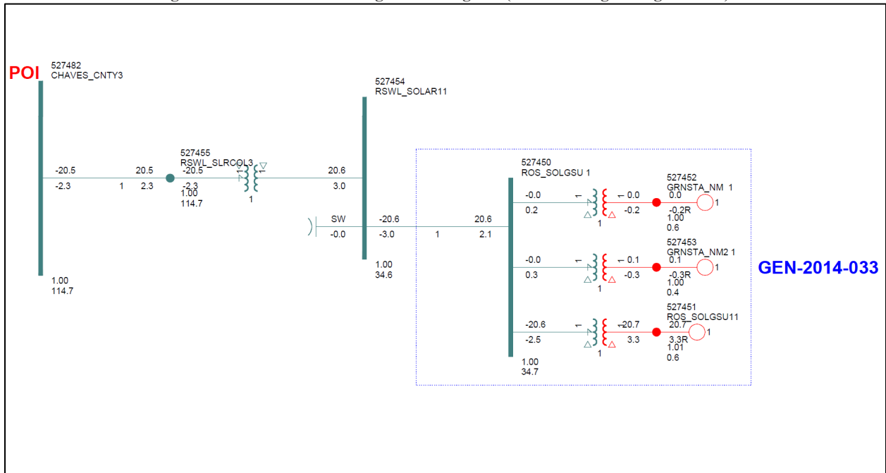
Figure 2-1: GEN-2014-033 Single Line Diagram (EGF Existing Configuration*)
