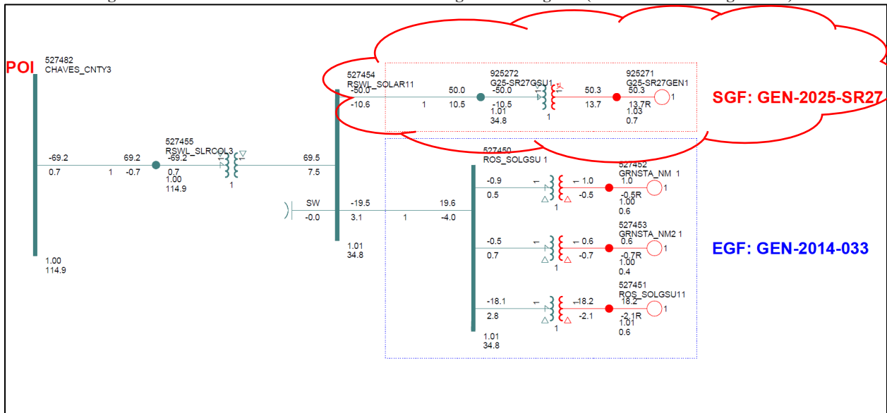
Figure 2-2: GEN-2014-033 & GEN-2025-SR27 Single Line Diagram (EGF & SGF Configuration)
