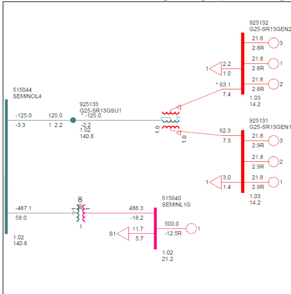
Figure 2-2: Seminole 138 kV Unit & GEN-2025-SR13 Single Line Diagram (EGF & SGF Configuration)
