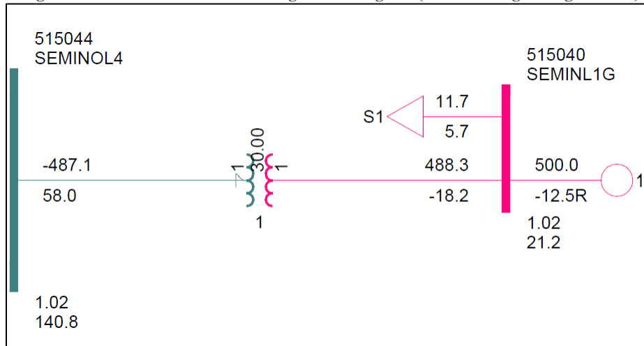
Figure 2-1: Seminole 138 kV Unit Single Line Diagram (EGF Existing Configuration*)
