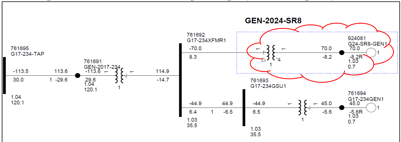
Figure 2-2: GEN-2017-234 & GEN-2024-SR8 Single Line Diagram (EGF & SGF Configuration)
