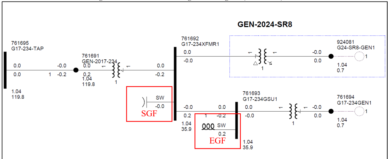
Figure 3-1: GEN-2024-SR8 Single Line Diagram (Shunt Sizes)
