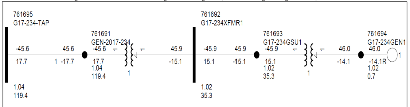
Figure 2-1: GEN-2017-234 Single Line Diagram (EGF Existing Configuration*)
