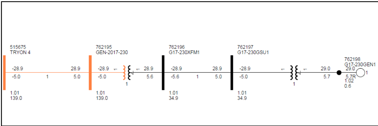
Figure 2-1: GEN-2017-230 Single Line Diagram (EGF Existing Configuration*)
