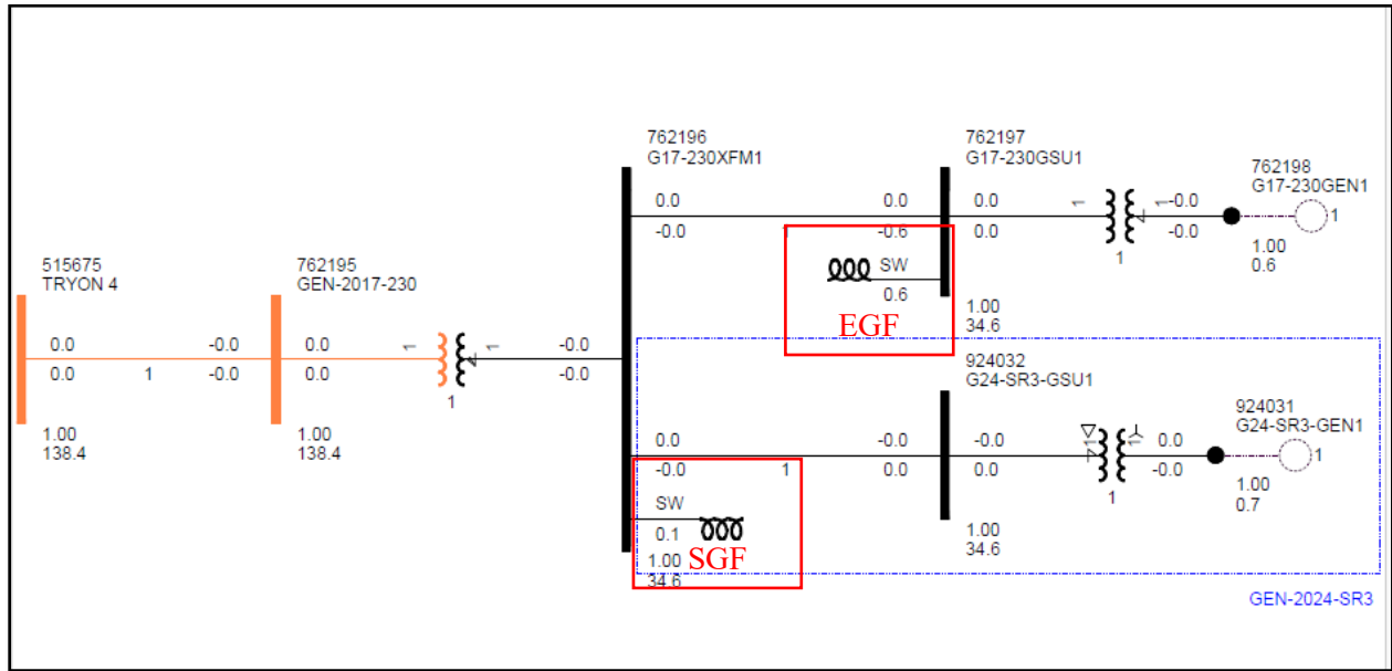
Figure 3-1: GEN-2024-SR3 Single Line Diagram (Shunt Sizes)
