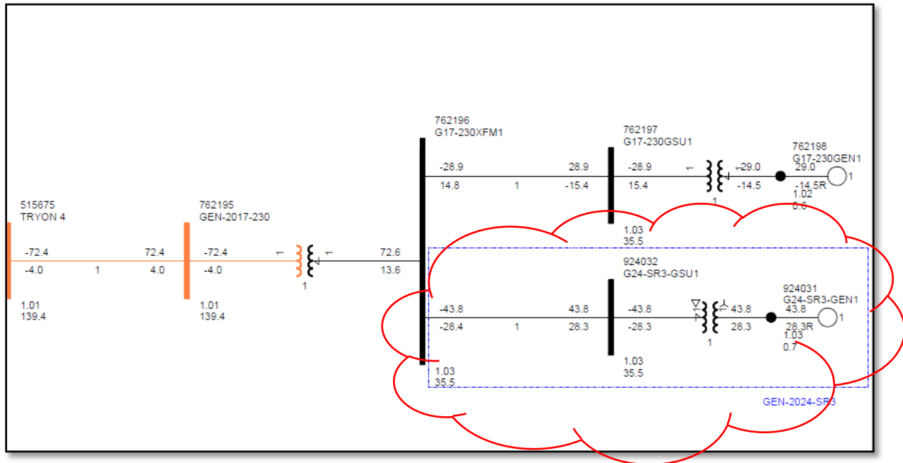
Figure 2-2: GEN-2017-230 & GEN-24-SR3 Single Line Diagram (EGF & SGF Configuration)
