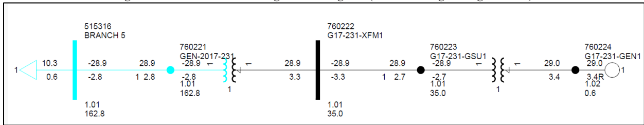
Figure 2-1: GEN-2017-231 Single Line Diagram (EGF Existing Configuration*)
