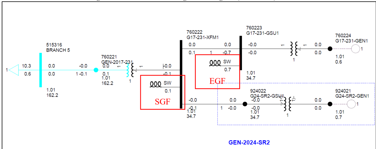
Figure 3-1: GEN-2024-SR2 Single Line Diagram (Shunt Sizes)
