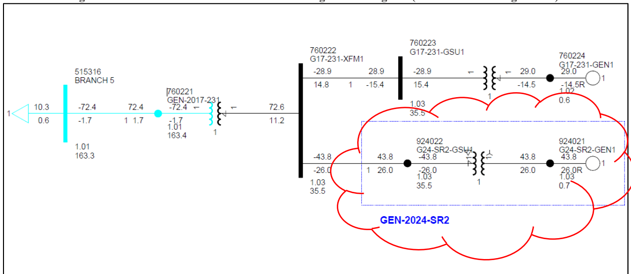
Figure 2-2: GEN-2017-231 & GEN-2024-SR2 Single Line Diagram (EGF & SGF Configuration)
