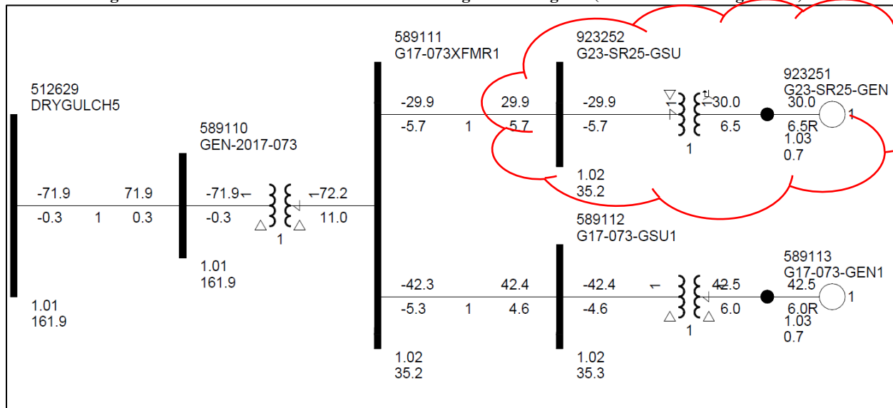
Figure 2-2: GEN-2017-073 & GEN-2023-SR25 Single Line Diagram (EGF & SGF Configuration)
