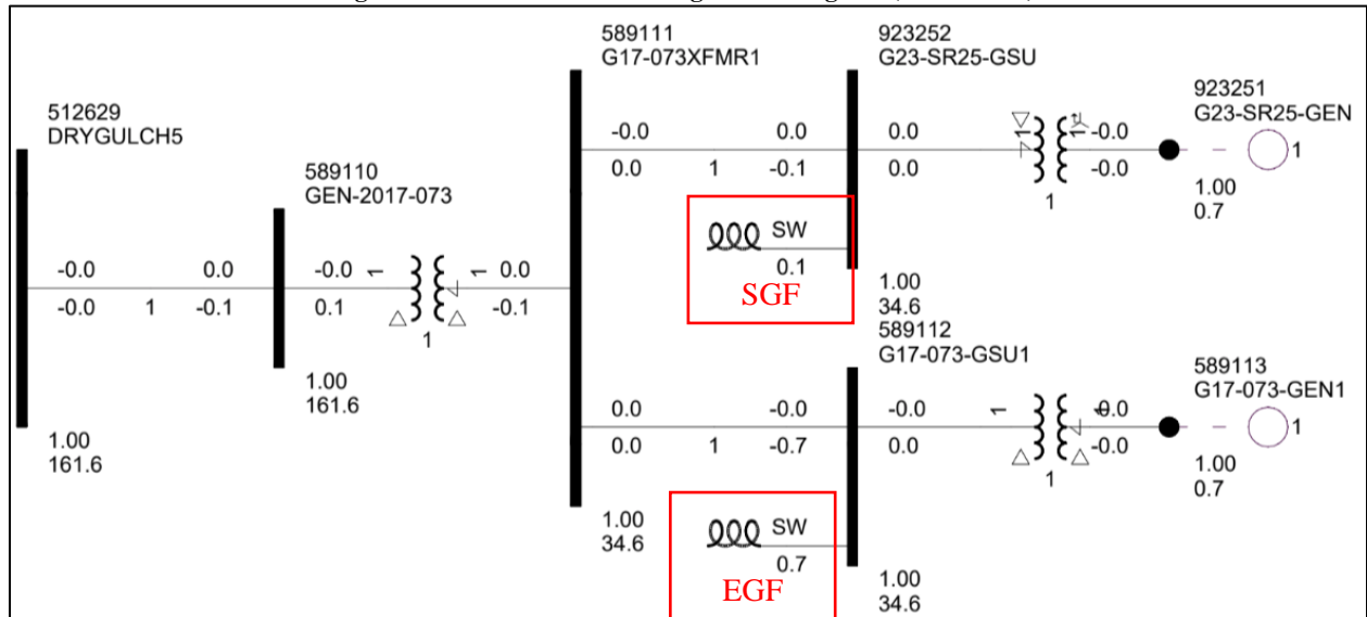
Figure 3-1: GEN-2023-SR25 Single Line Diagram (Shunt Sizes)
