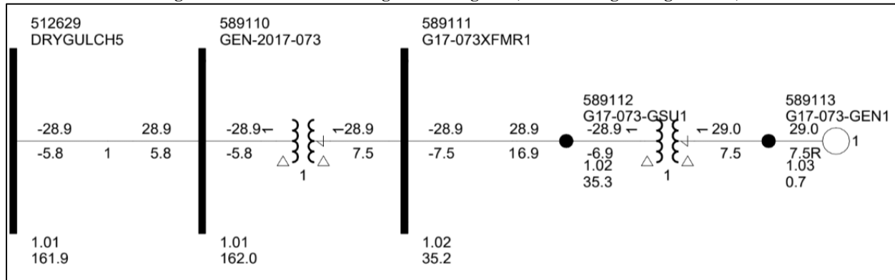
Figure 2-1: GEN-2017-073 Single Line Diagram (EGF Existing Configuration*)
