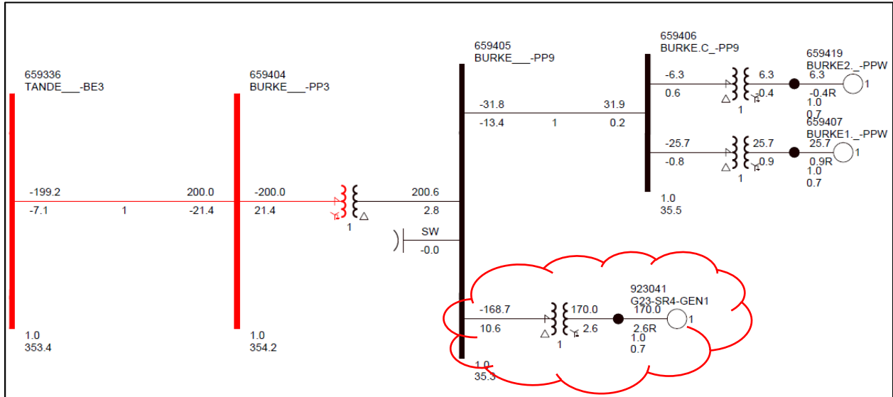
Figure 2-2: GEN-2016-151 & GEN-2023-SR4 Single Line Diagram (EGF & SGF Configuration)
