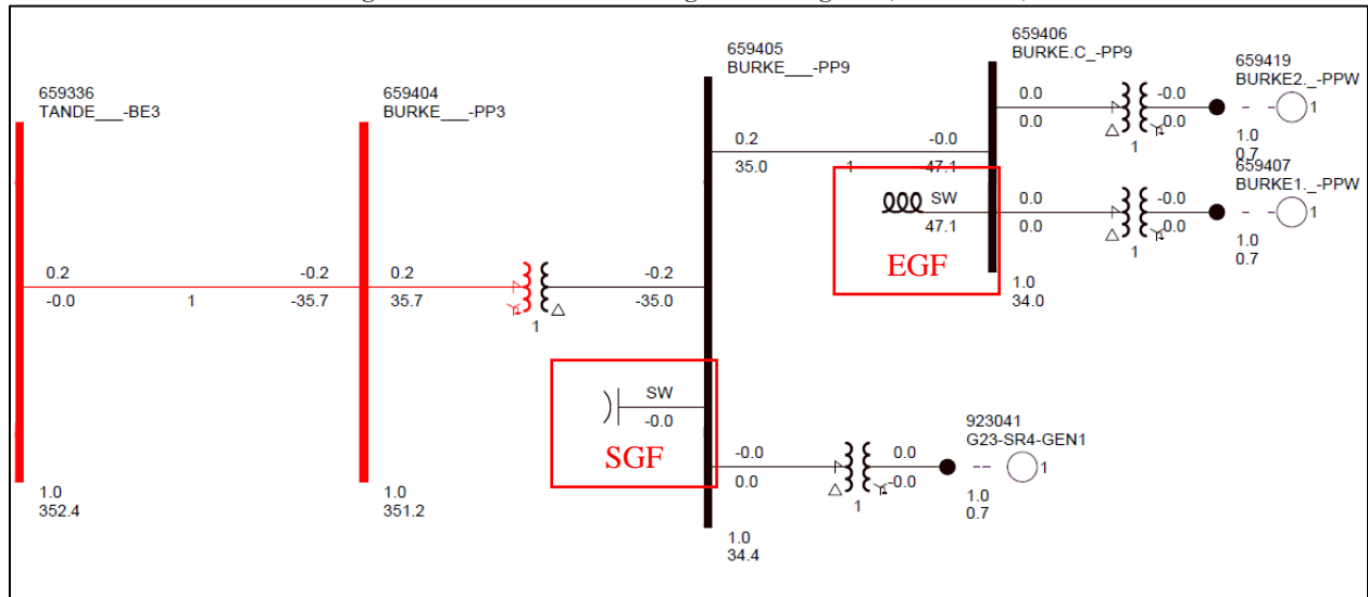
Figure 3-1: GEN-2023-SR4 Single Line Diagram (Shunt Sizes)
