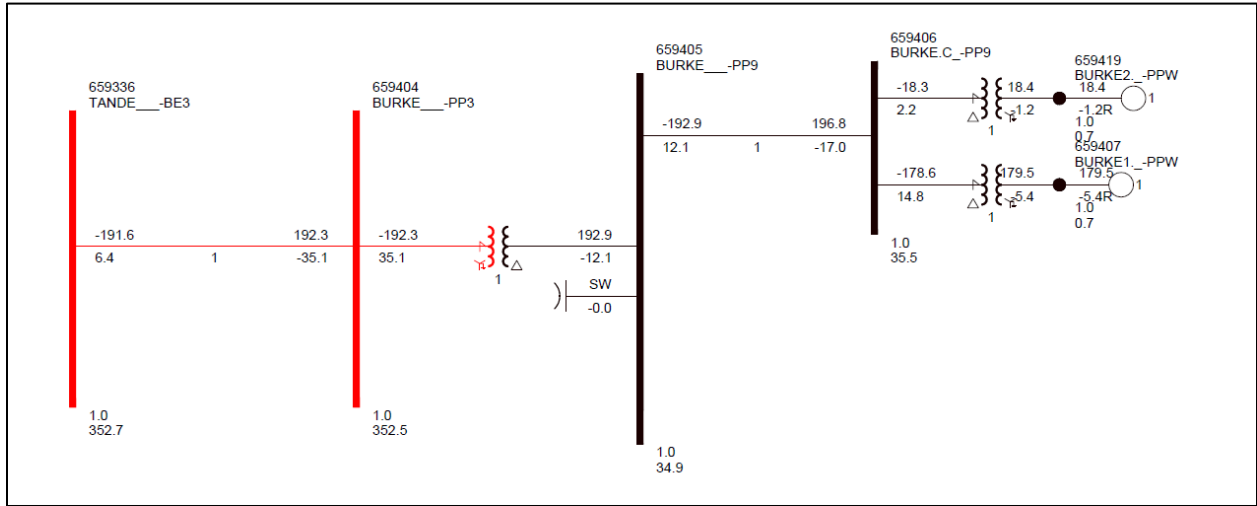
Figure 2-1: GEN-2016-151 Single Line Diagram (EGF Existing Configuration*)
