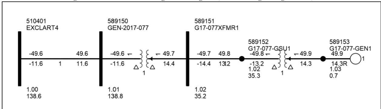
Figure 2-1: GEN-2017-077 Single Line Diagram (EGF Existing Configuration*)
