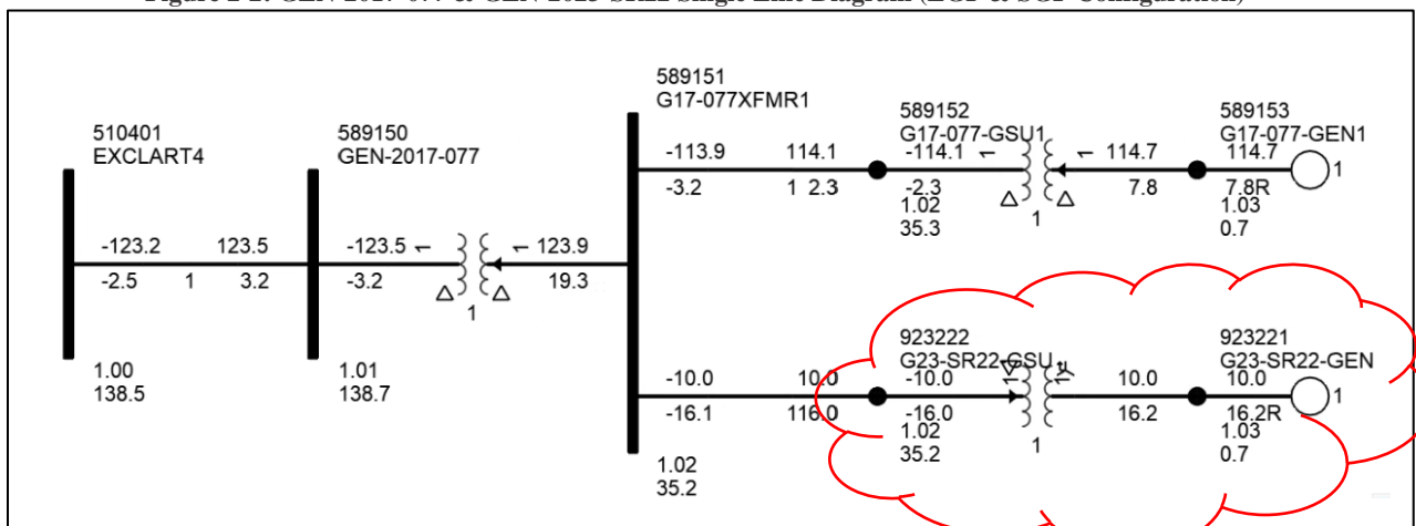
Figure 2-2: GEN-2017-077 & GEN-2023-SR22 Single Line Diagram (EGF & SGF Configuration)
