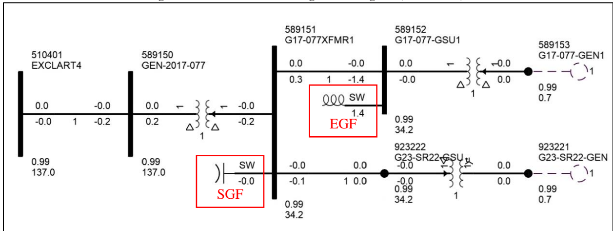
Figure 3-1: GEN-2023-SR22 Single Line Diagram (Shunt Sizes)
