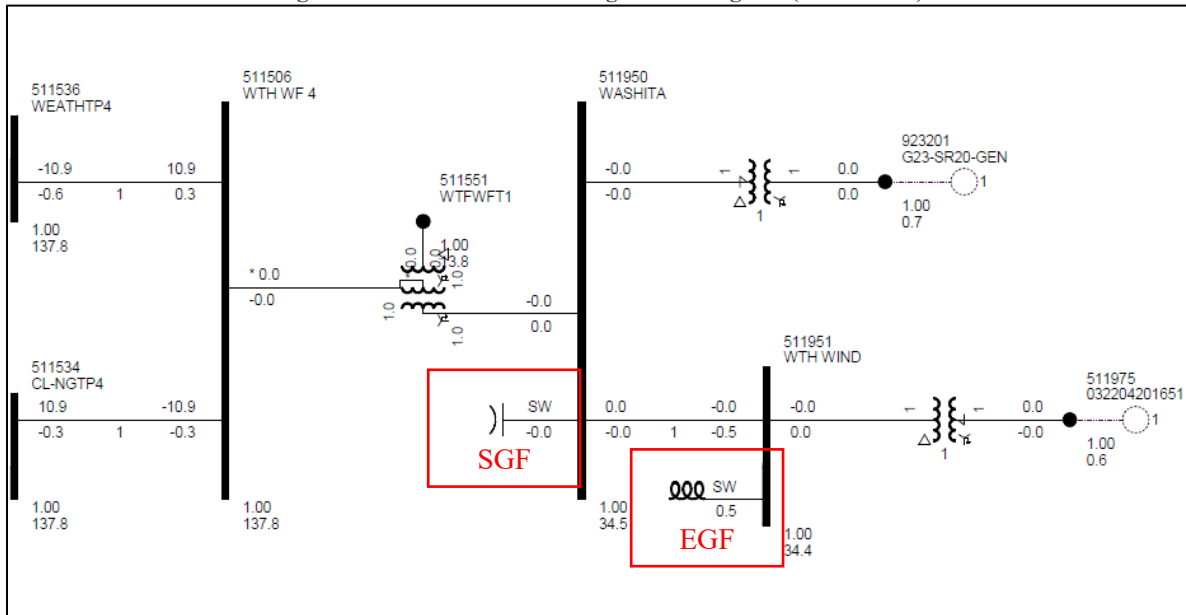
Figure 3-1: GEN-2023-SR20 Single Line Diagram (Shunt Sizes)
