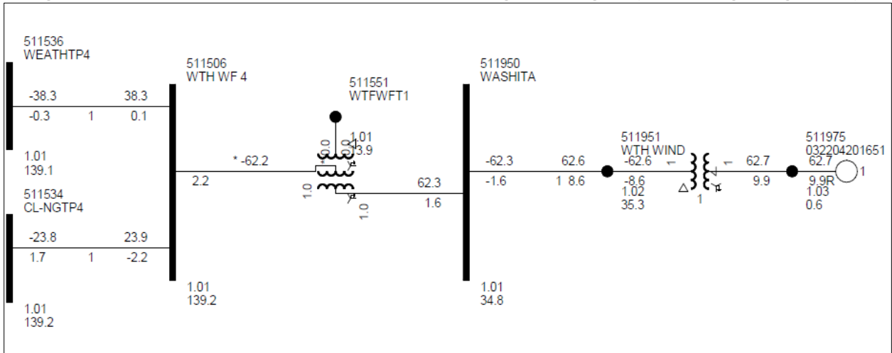
Figure 2-1: GEN-2003-022, GEN-2004-020, & GEN-2016-051 Single Line Diagram (EGF Existing Configuration*)
