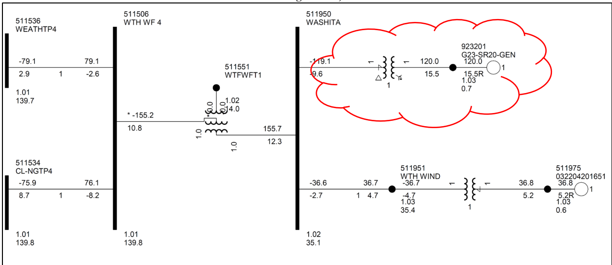
Figure 2-2: GEN-2003-022, GEN-2004-020, & GEN-2016-051 & GEN-2023-SR20 Single Line Diagram (EGF & SGF Configuration)
