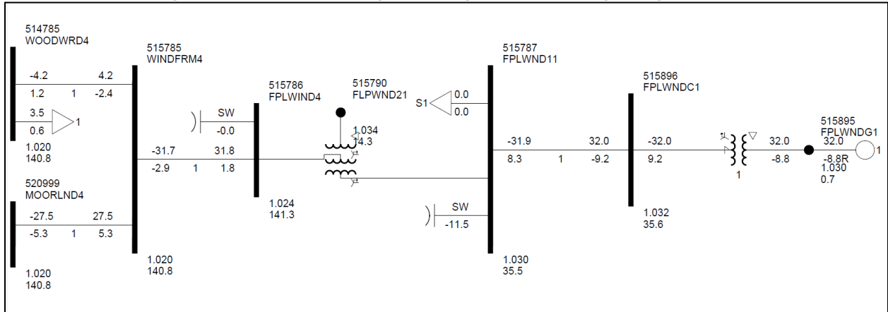
Figure 2-1: GEN-2001-037 Single Line Diagram (EGF Existing Configuration*)
