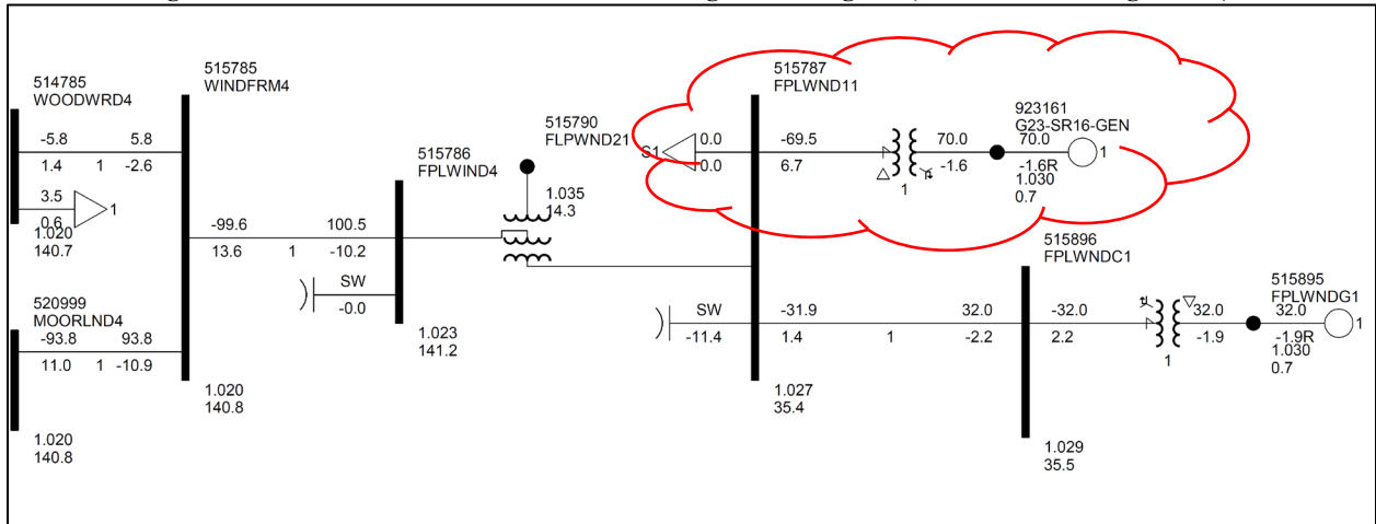
Figure 2-2: GEN-2001-037 & GEN-2023-SR16 Single Line Diagram (EGF & SGF Configuration)
