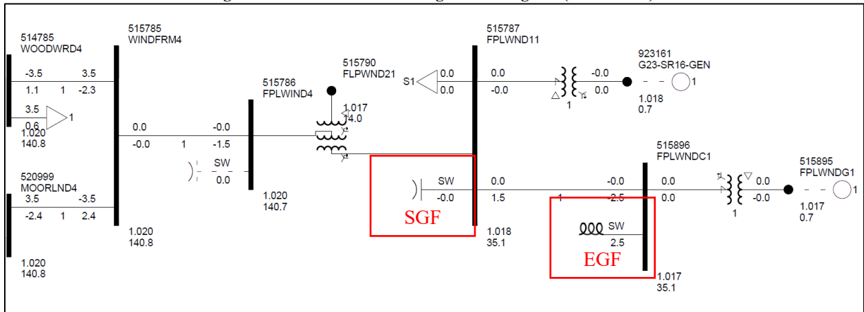
Figure 3-1: GEN-2023-SR16 Single Line Diagram (Shunt Sizes)
