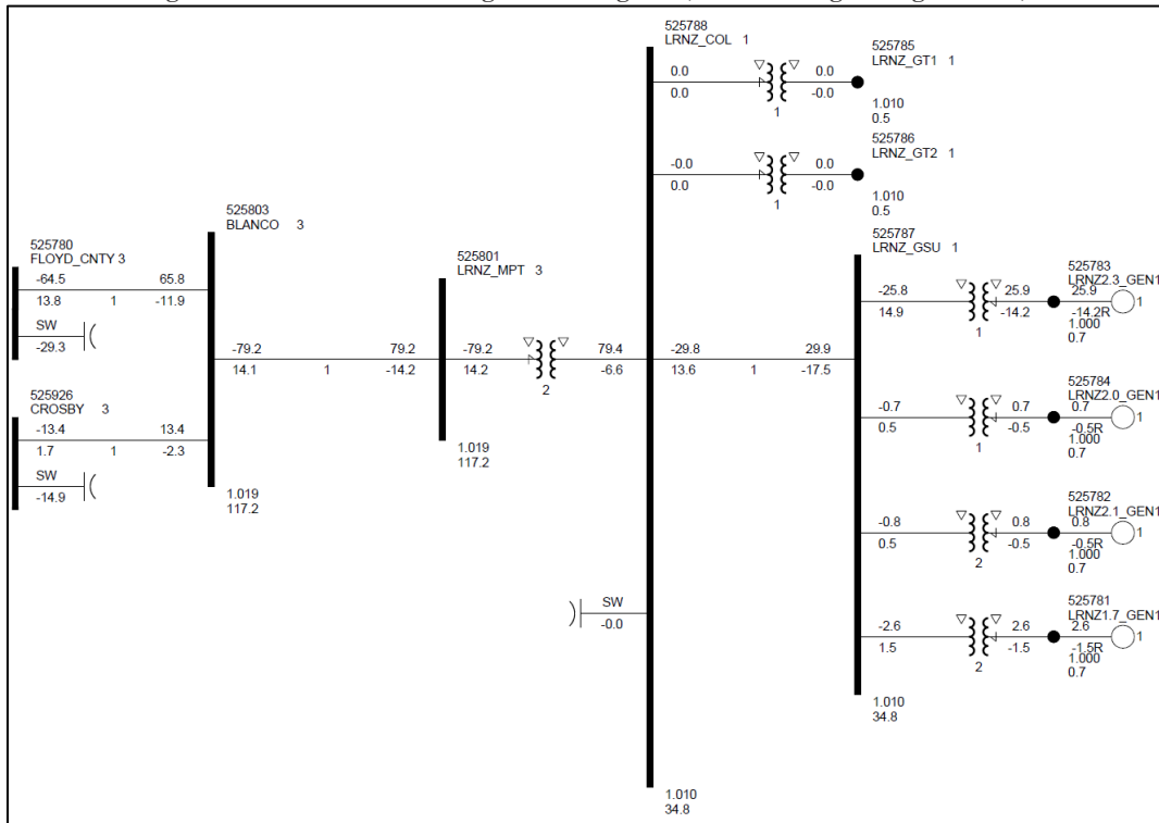
Figure 2-1: GEN-2011-025 Single Line Diagram (EGF Existing Configuration*)
