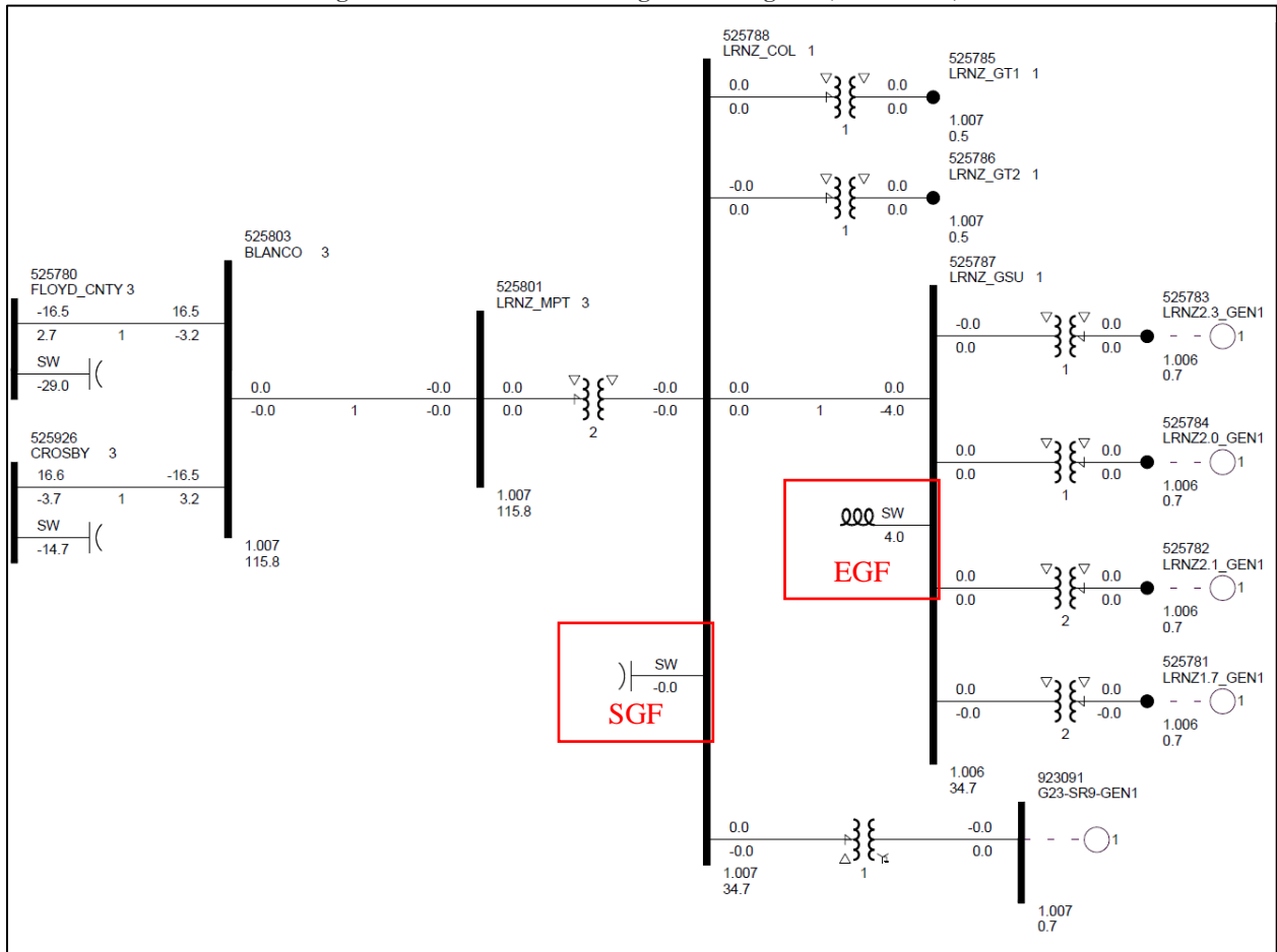
Figure 3-1: GEN-2023-SR9 Single Line Diagram (Shunt Sizes)
