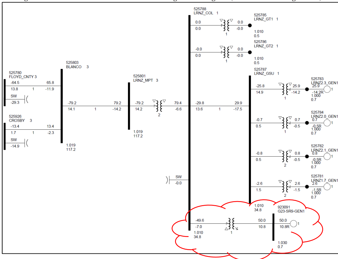
Figure 2-2: GEN-2011-025 & GEN-2023-SR9 Single Line Diagram (EGF & SGF Configuration)
