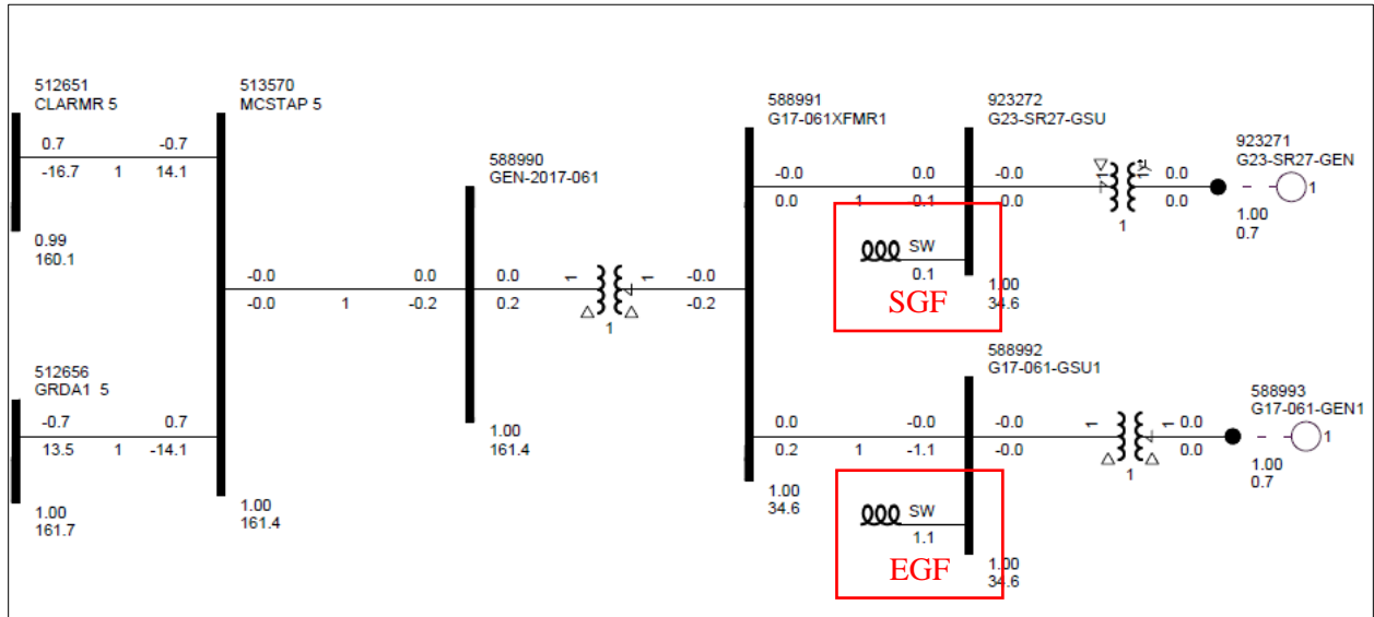
Figure 3-1: GEN-2023-SR27 Single Line Diagram (Shunt Sizes)
