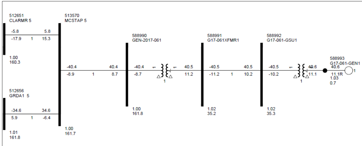
Figure 2-1: GEN-2017-061 Single Line Diagram (EGF Existing Configuration*)
