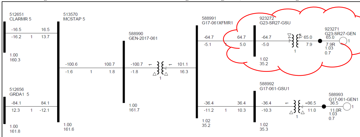
Figure 2-2: GEN-2017-061 & GEN-2023-SR27 Single Line Diagram (EGF & SGF Configuration)
