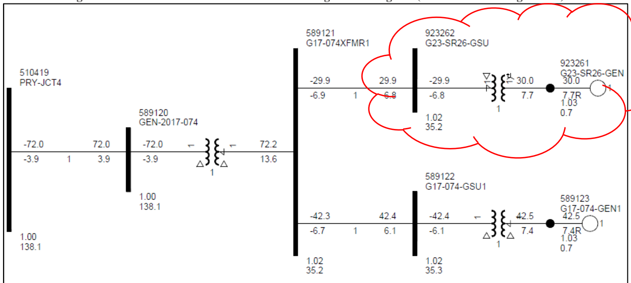
Figure 2-2: GEN-2017-074 & GEN-2023-SR26 Single Line Diagram (EGF & SGF Configuration)
