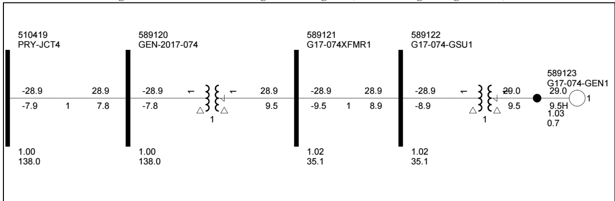
Figure 2-1: GEN-2017-074 Single Line Diagram (EGF Existing Configuration*)
