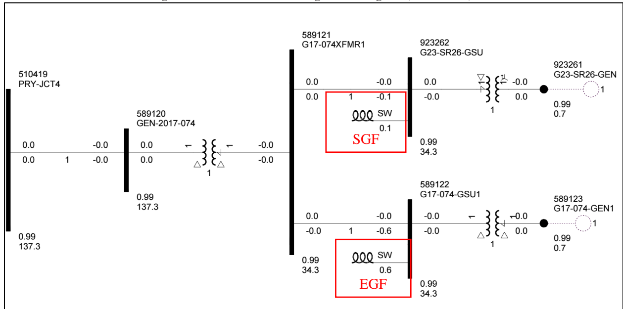
Figure 3-1: GEN-2023-SR26 Single Line Diagram (Shunt Sizes)
