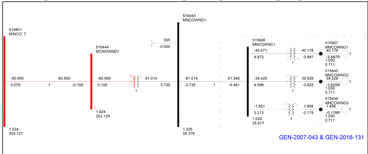
Figure 2-1: GEN-2007-043 & GEN-2016-131 Single Line Diagram (EGF Existing Configuration*)
