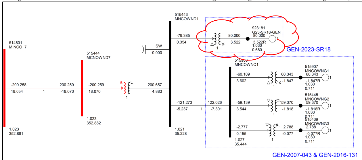
Figure 2-2: GEN-2007-043 & GEN-2016-131 & GEN-2023-SR18 Single Line Diagram (EGF & SGF Configuration)
