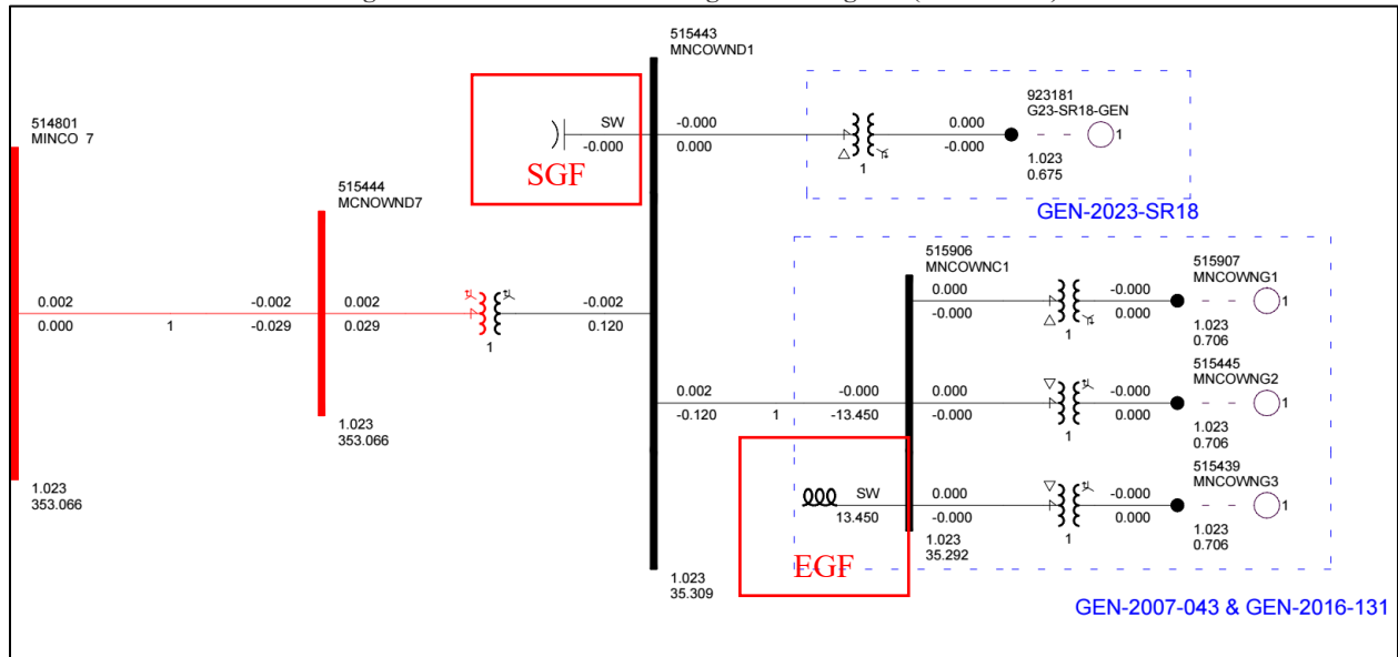
Figure 3-1: GEN-2023-SR18 Single Line Diagram (Shunt Sizes)
