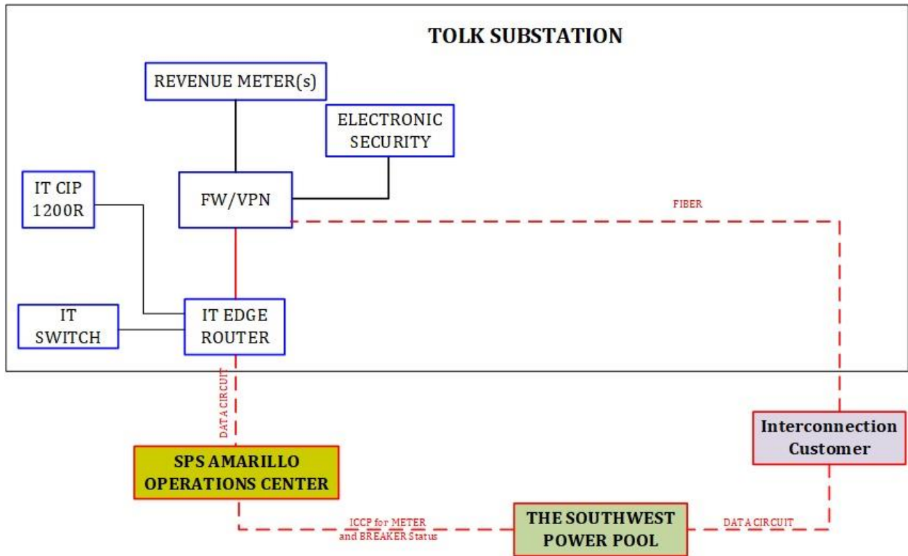
Figure 2 – Tolk Station Communication Information
