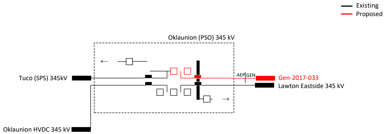
Figure 1: Point of Interconnection (POI INFORMATION) One-Line Diagram
