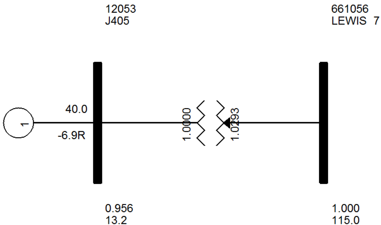
Figure 1: Proposed POI Configuration and Request Power Flow Model
