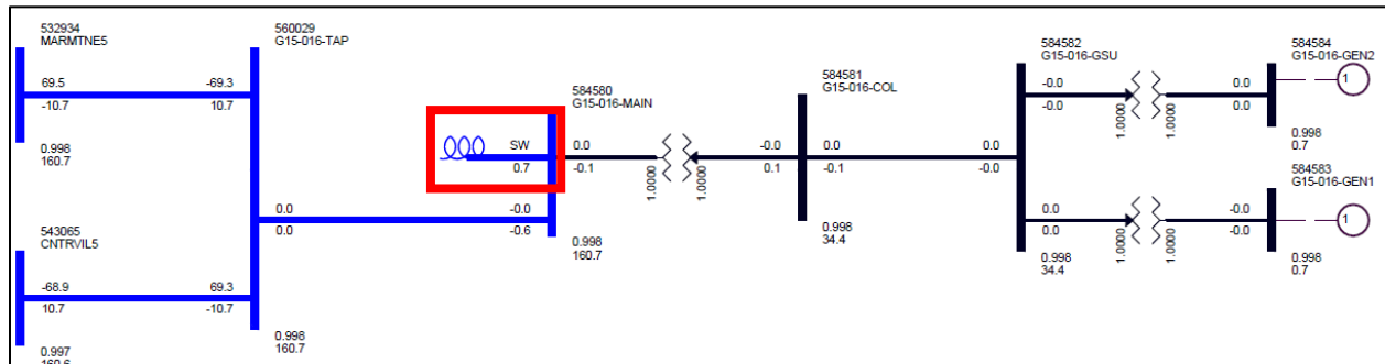
FIGURE D-1: GEN-2015-016 WITH GENERATION OFF AND SHUNT REACTOR
