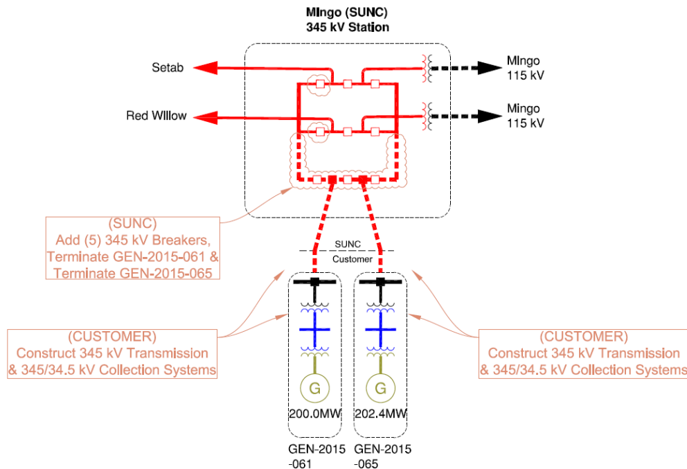
Figure 1: Interconnection Configuration for GEN-2015-065
