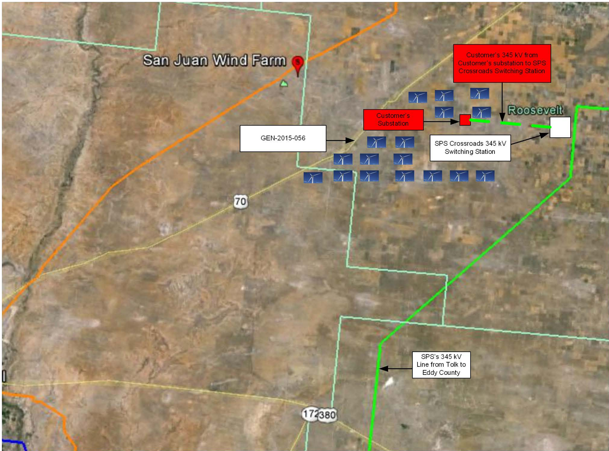
Figure A-1. Approximate location of Crossroads Switching Station and IC's Wind Farm
