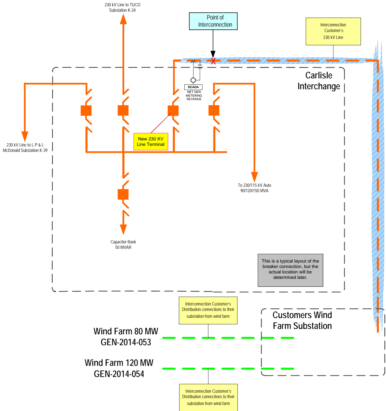
Figure A-1. One-line Diagram of Carlisle Interchange
