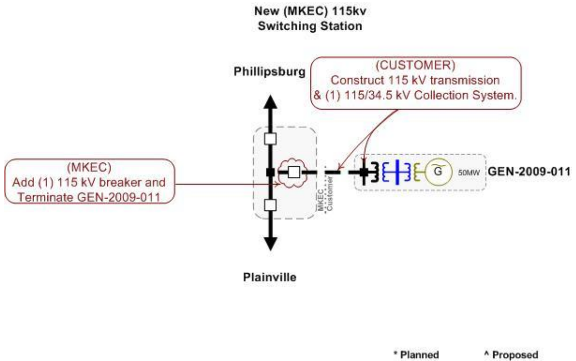
Figure 1: GEN-2009-011 Facility and Proposed Interconnection Configuration
