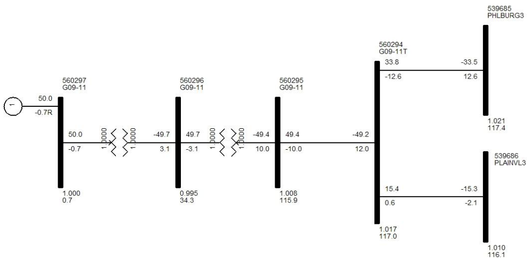
Figure 2: GEN-2009-011 Bus Interconnection
